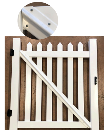
Step 6: Cut cross bar to desired length & make sure it's attached at the top of the hinge side. Step 7: Install Hinges and Latch per directions in hardware package. (Sold Separately)
